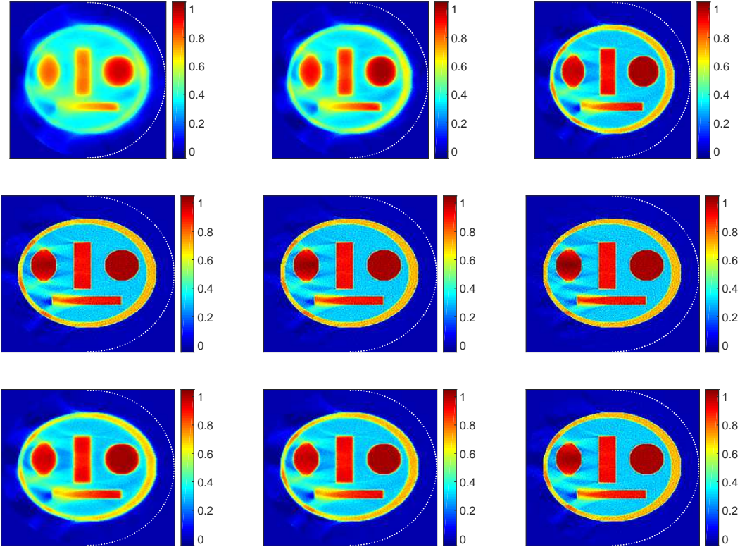
Figure 3.3: Reconstructions from exact data after 10 iterations (left), 20 iterations (center) and 80 iterations (right). Top row: Landweber. Middle row: Kaczmarz. Bottom row: AVEK.
