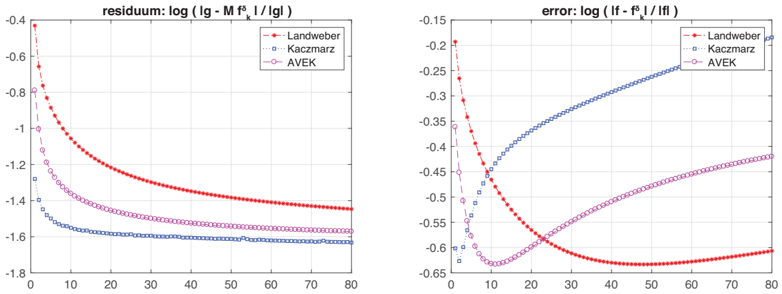
Figure 3.4: Residuum and relative reconstruction error (after taking logarithm to basis 10) for noisy data during the first 80 cycles. One notices the typical semi convergence behavior of all methods.
