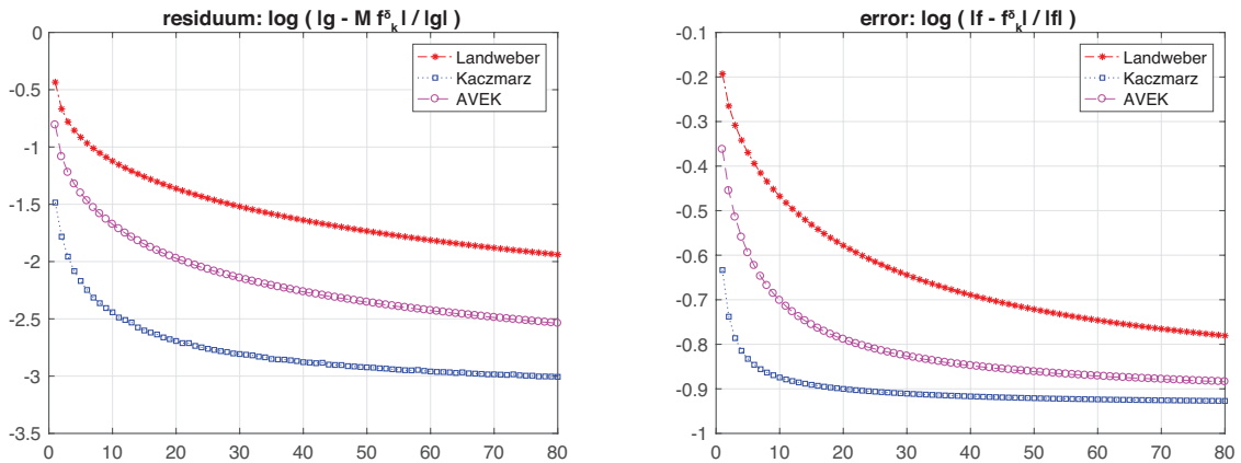
Figure 3.2: Residuum and relative reconstruction error (after taking logarithm to basis 10) for exact data during the first 80 cycles.
