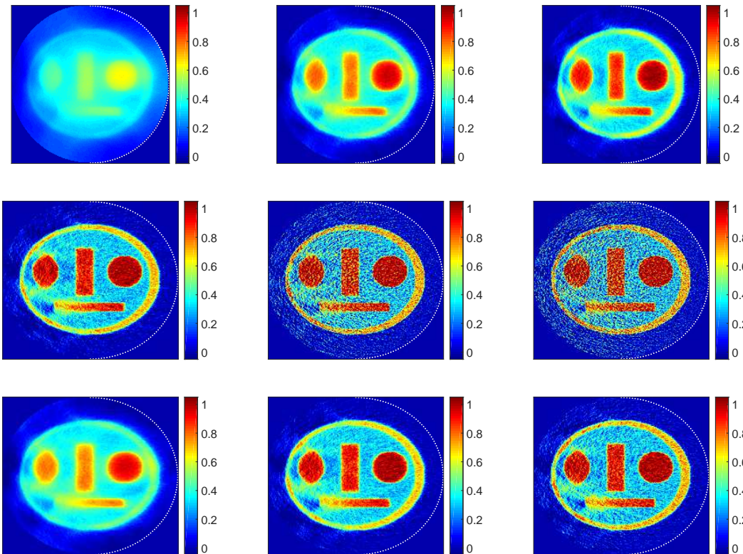
Figure 3.5: Reconstructions from noisy data after 2 iterations (left), 10 iterations (center) and 20 iterations (right). Top row: Landweber. Middle row: Kaczmarz. Bottom row: AVEK.
