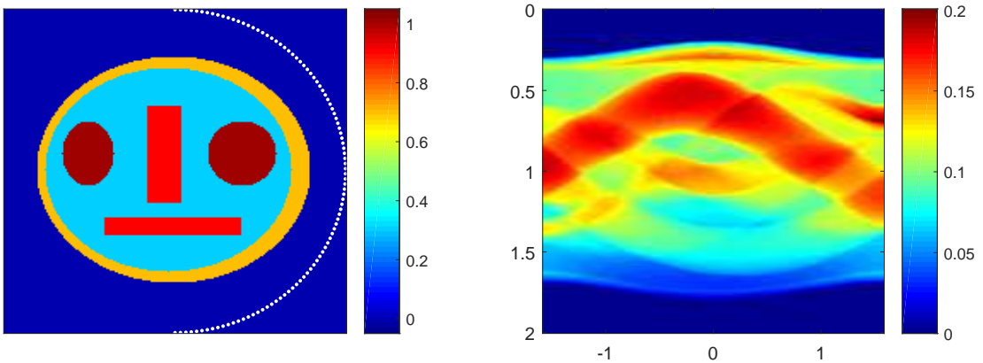
Figure 3.1: Left: The phantom \mathbf{f} \in \mathbb{R}^{201 \times 201} discretizing the head like function supported in a disc of radius 1. The white dots indicate locations of detectors. Right: The simulated discrete circular Radon transform \mathbf{g} \in \mathbb{R}^{100 \times 201} . The horizontal axis is the detector location in [-\pi/2, \pi/2] ; the vertical axis the radius in [0, 2] . Any partial data \mathbf{g}_i \in \mathbb{R}^{1 \times 201} corresponds to a column.
